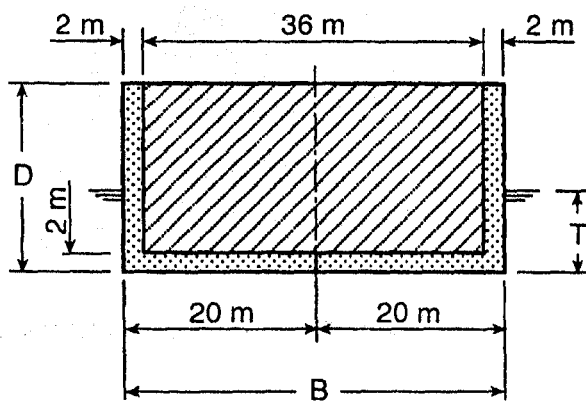
Midship section
