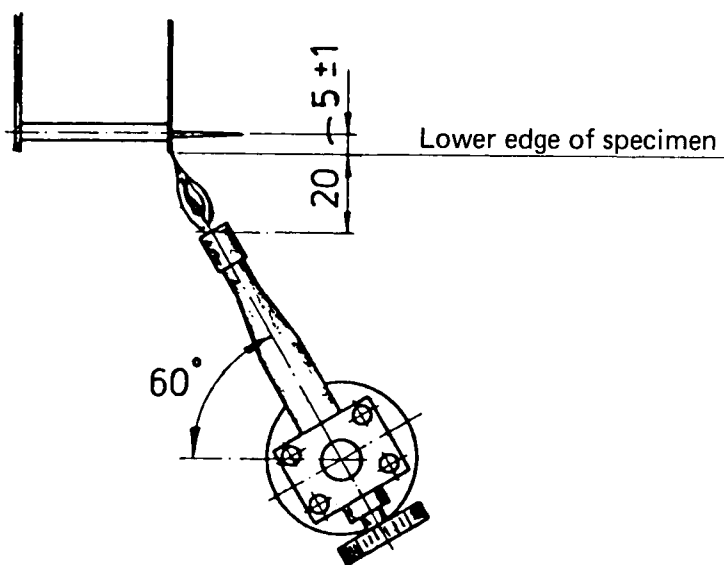
Figure 2 — Ignition burner — Fabric positions
